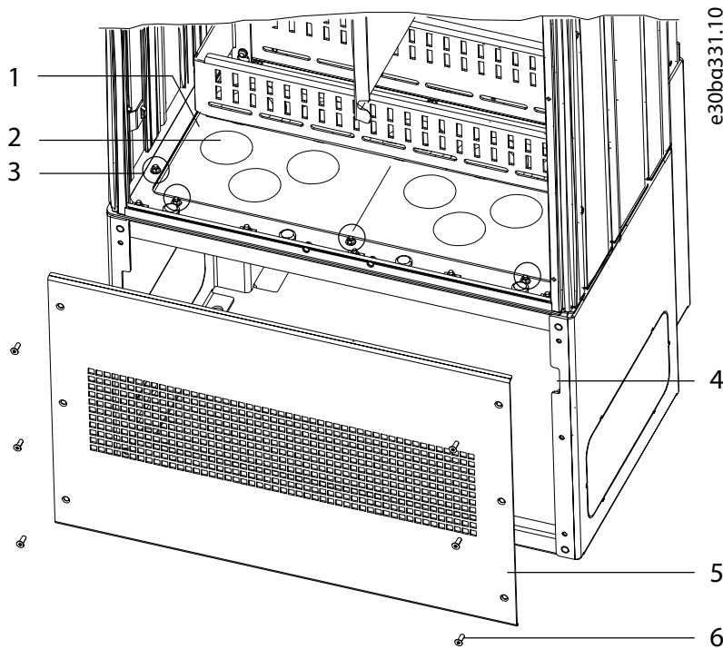
Illustration 5: Cable Entry Plate Installation
