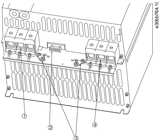
Ilustracija 7: Velikost ohišja H8, IP20, 380–480 V, 90 kW (125 KM), IP20, 200–240 V, 37–45 kW (50–60 KM), IP20, 525–600 V, 75–90 kW (100–125 KM)
