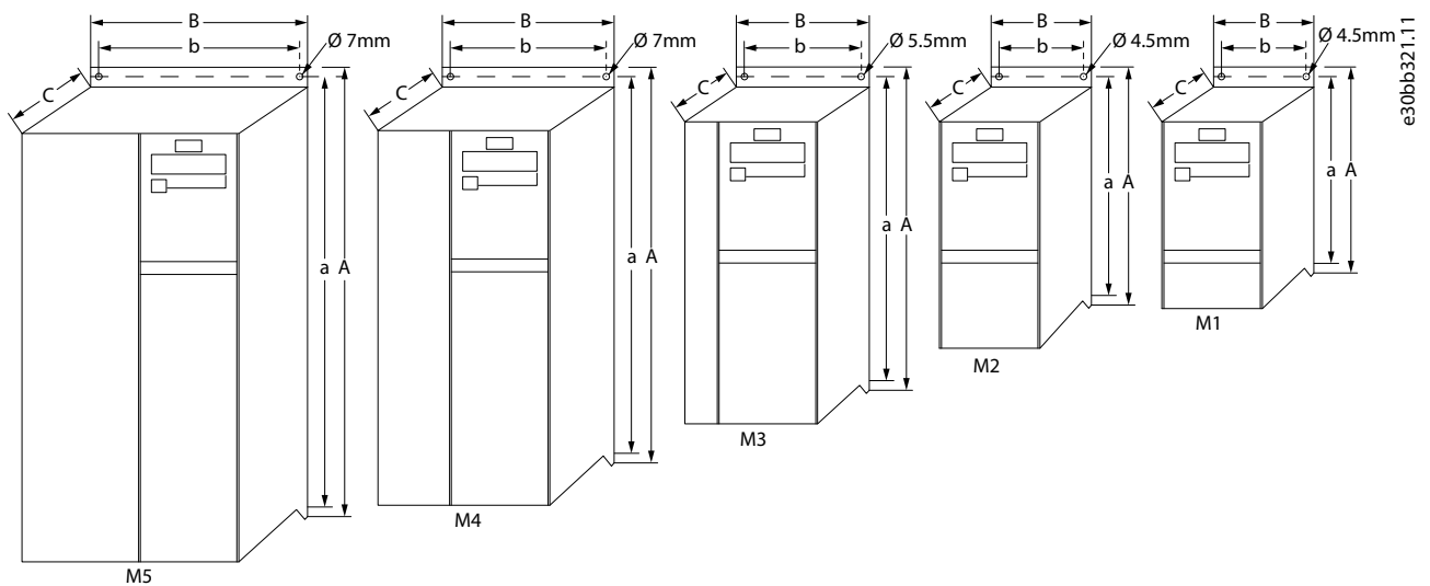
Illustration 1: Mechanical Dimensions
