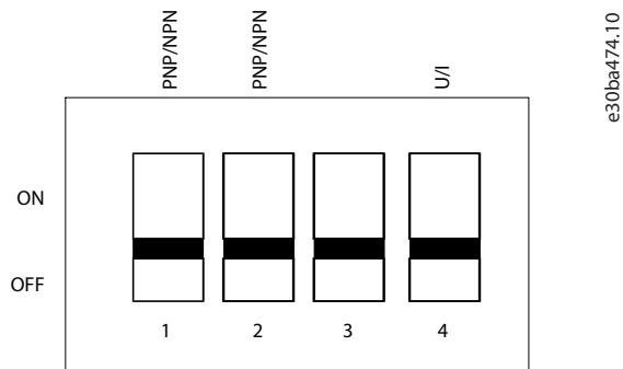
Illustration 4: S200 Switches 1–4
