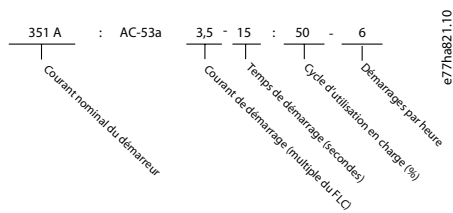
Illustration 3: Format AC53a (courant nominal sans bipasse)
