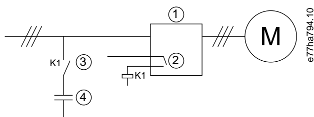
Illustration 6: Schéma de raccordement
