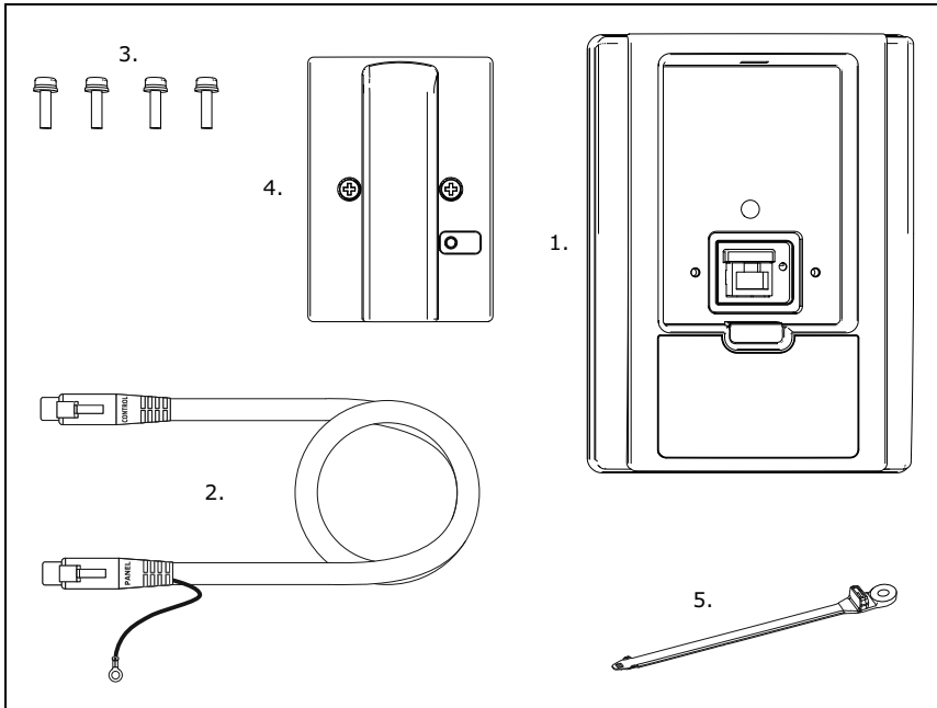
Figure 1. Door keypad mounting kit
