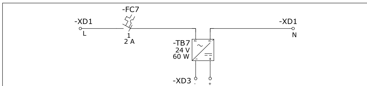
Fig. 20: Alimentation 24 Vc.c.
