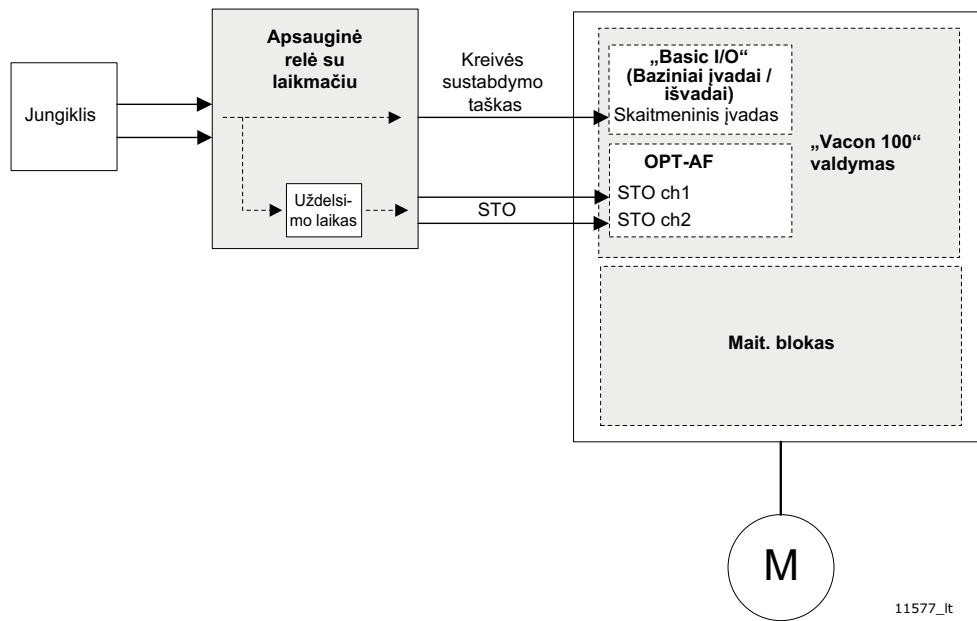
8 pav. 1 saugaus sustabdymo prijungimo principas (SS1)
