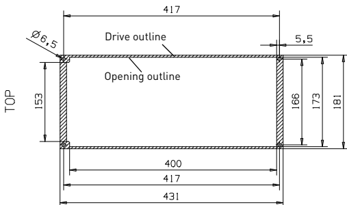
Figure 6: Flange mounting cutout dimensions for MI5 (Unit: mm)
