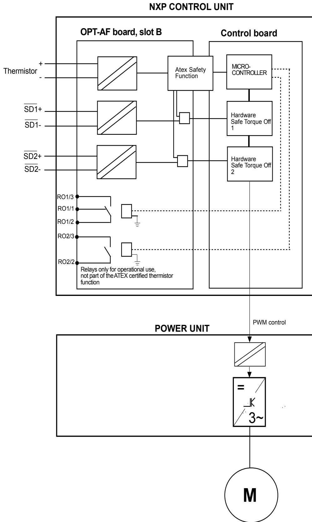
Figure 16. Thermistor function principle in NXP frequency converter with the OPT-AF board
