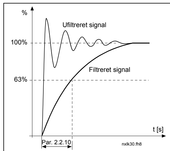
Figur 1- 3. AI-signalfiltrering
