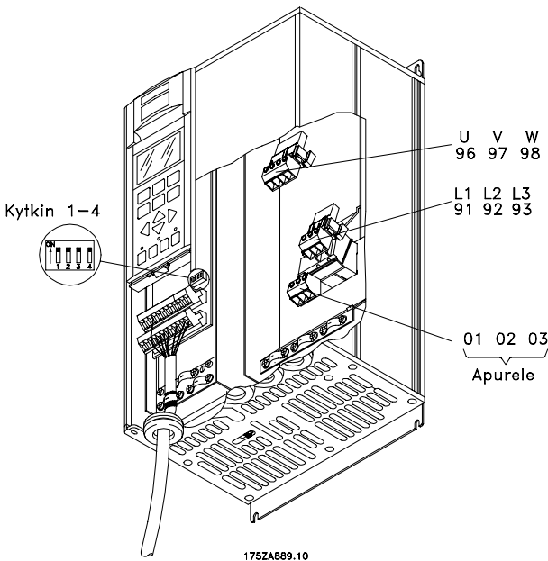
Compact IP 20/NEMA 1 VLT 8006-8011, 380-480 V VLT 8002-8011, 525-600 V
