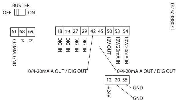
Illustration 1.4 Control Terminals
