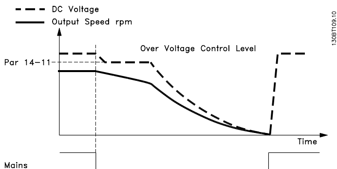
图 2.12: Kinetic Back-up, longer mains failure. The motor is coasted as soon as the energy in the system is too low.
