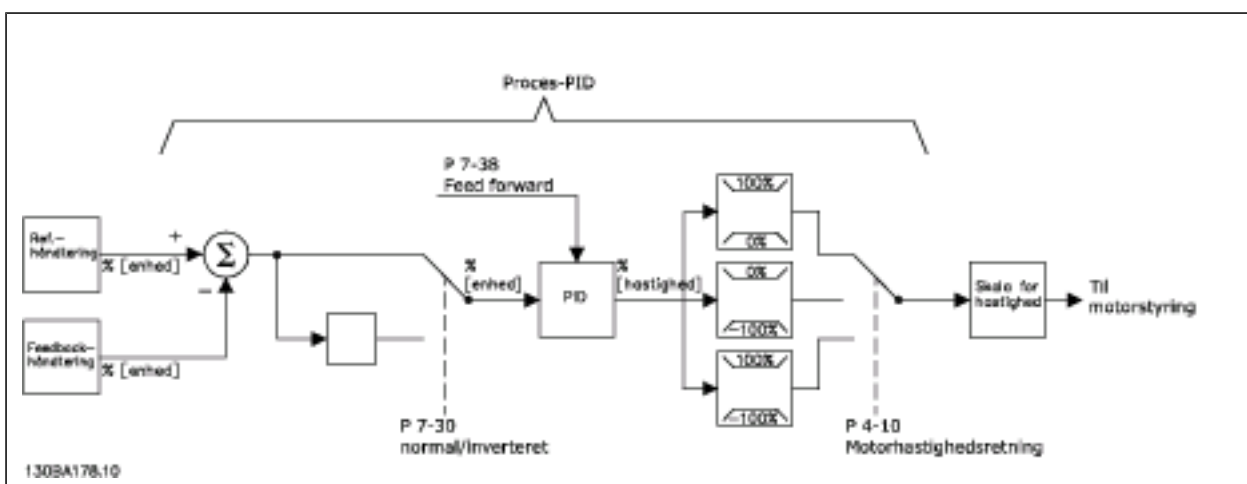
Diagram over Proces, PID-styring
