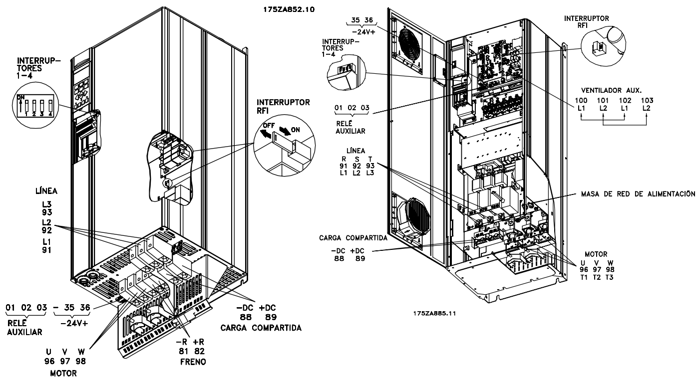
Compact IP 20 VLT 5072-5102 380-500 V
