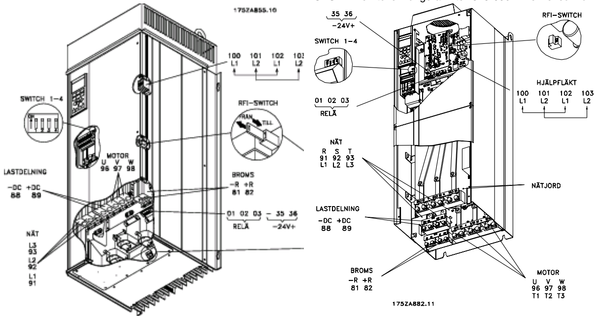
Compact IP 54 VLT 5072-5102 380-500 V
