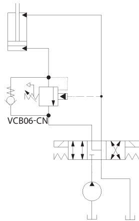
Load Holding - Single Actuator
