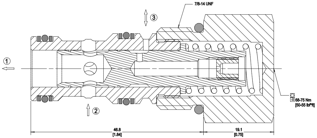
Compensated Bi-directional Flow Control
