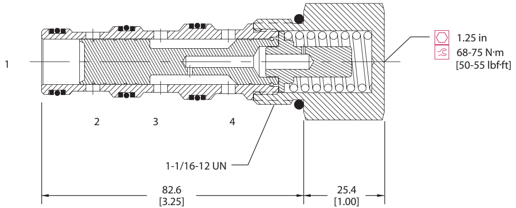
Cross-sectional view
