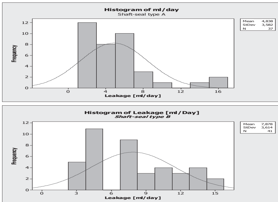
Figure 1: Histograms of Leakage for 2 different shaft seal types, where Leakage \llcorner 0
