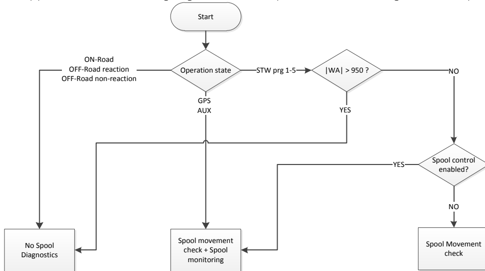
Figure 3 EHPS spool monitoring and spool movement check
