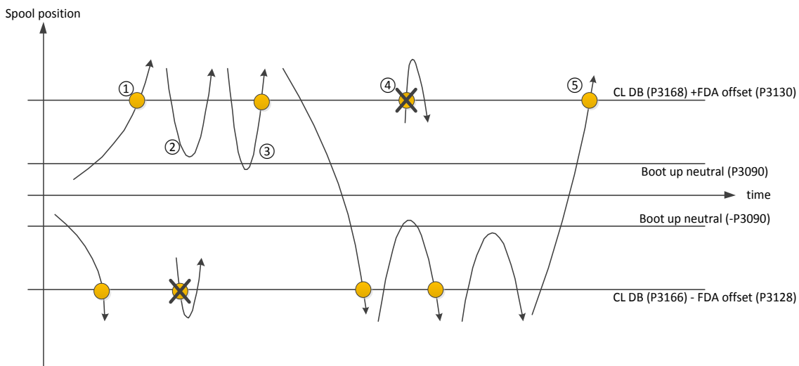
Figure 2 Spool movement check (EHPS)
