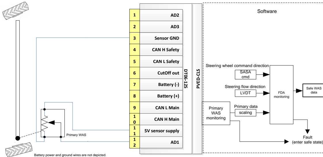
Figure 8 Single channel WAS sub-system (with FDA)
