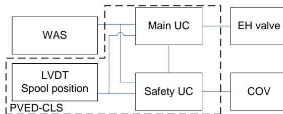
Figure 9 Single channel WAS interface with FDA monitoring
