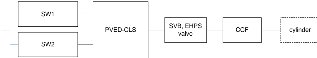
Figure 7 Safety related block diagram
