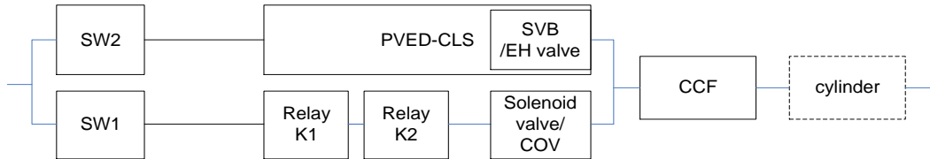
Figure 6 Safety related block diagram
