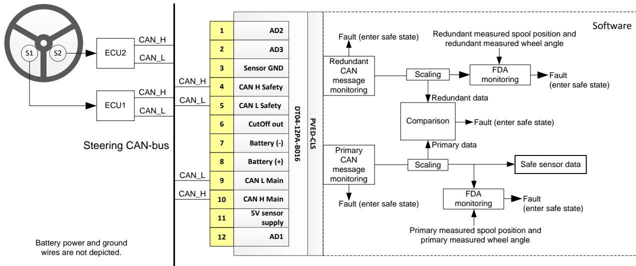
Figure 1: Mini-steering wheel architecture.
