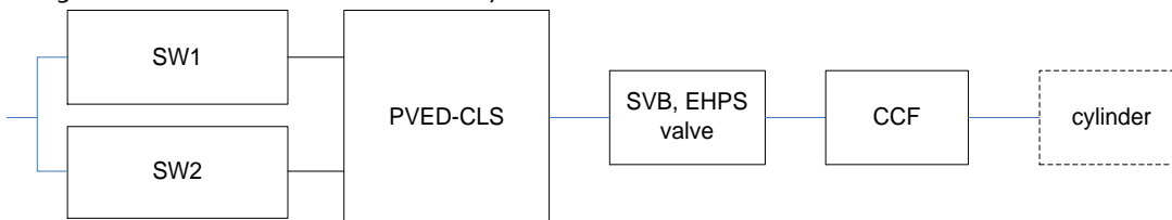
Figure 11 Safety related block diagram
