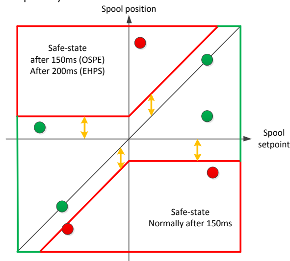
Figure 5 Spool monitoring
