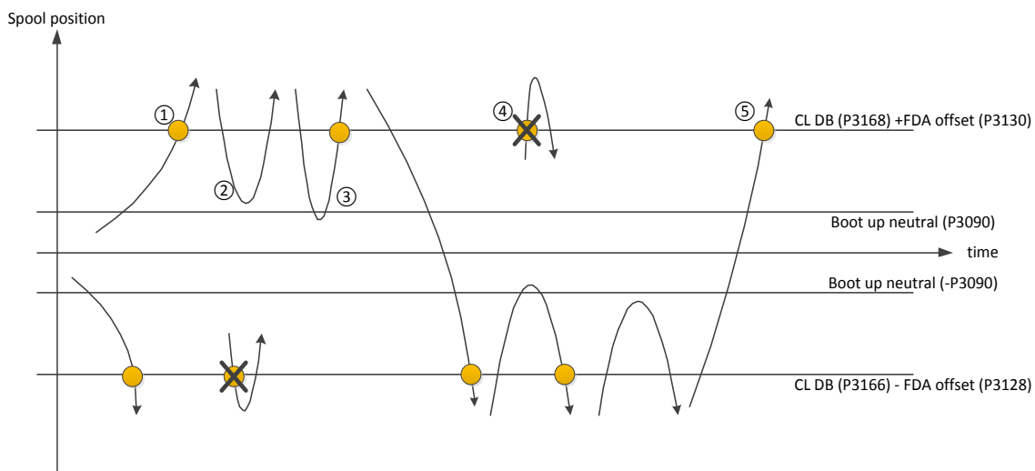
Figure 6 Spool movement check (EHPS)
