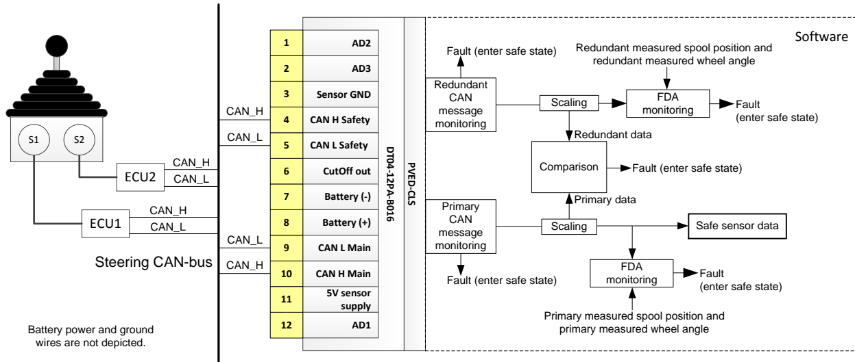
Figure 2: CAN based open-loop joystick architecture.
