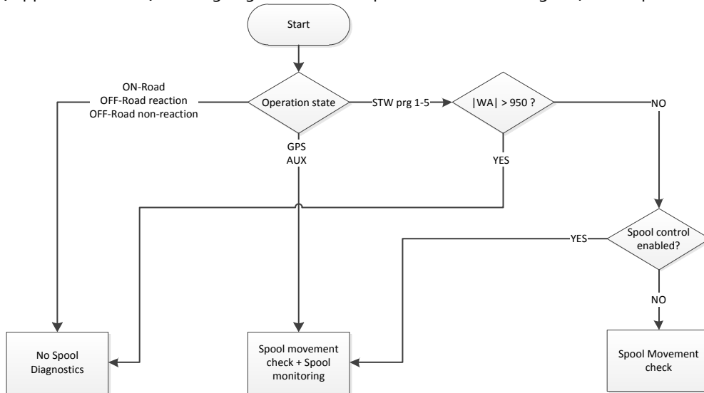
Figure 7 EHPS spool monitoring and spool movement check
