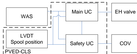
Figure 13 Single channel WAS interface with FDA monitoring
