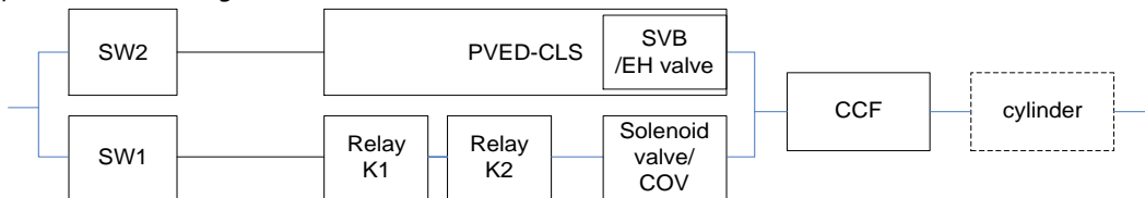
Figure 10 Safety related block diagram
