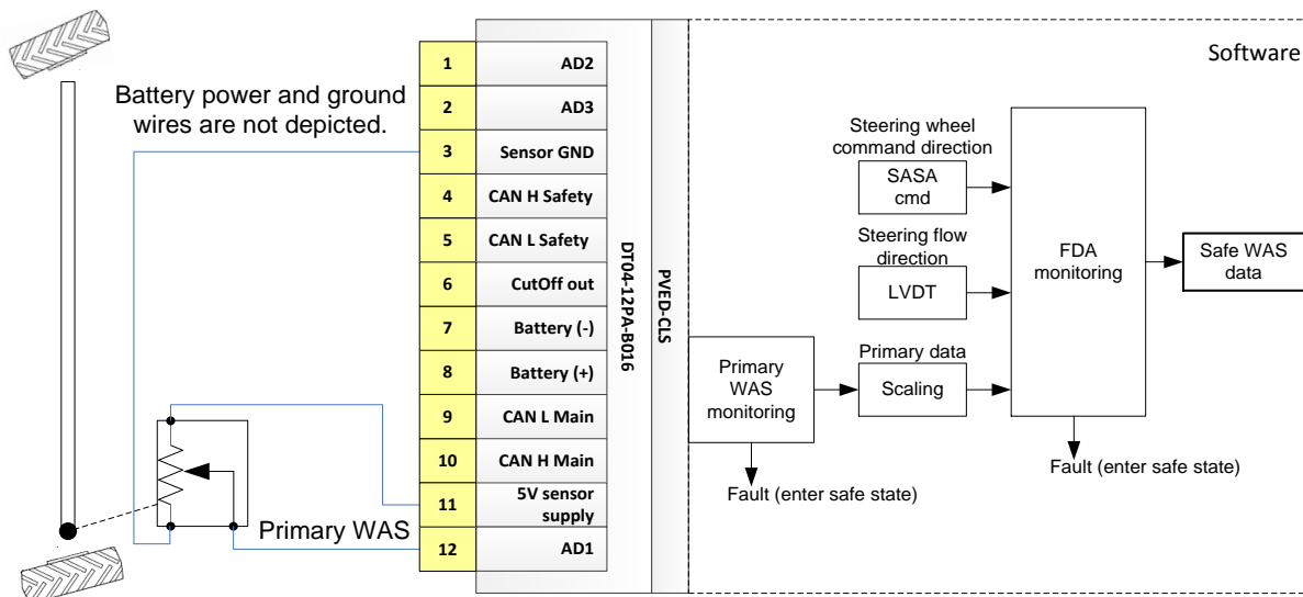
Figure 12 Single channel WAS sub-system (with FDA)
