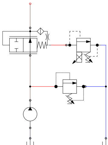
Pilot-Operated Pressure Reducing Valve
