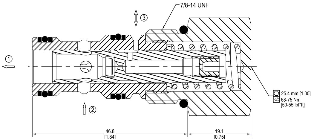
Cross-sectional view
