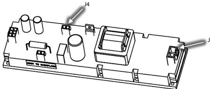
Figure 4 – Potted DC-DC Converter J1 and J4 Locations
