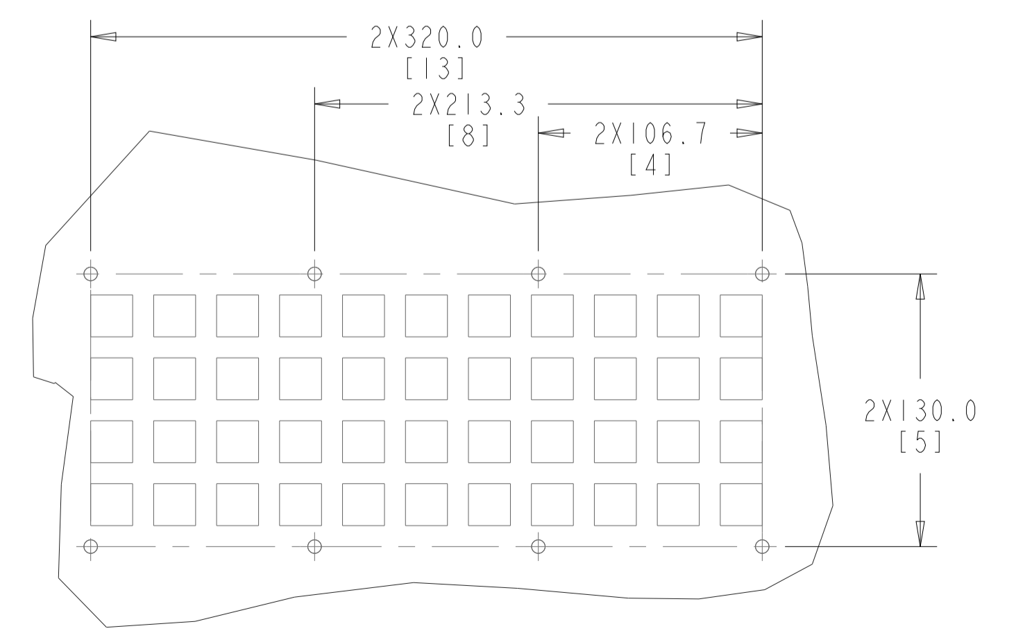
DETAIL B SCALE 0.400
