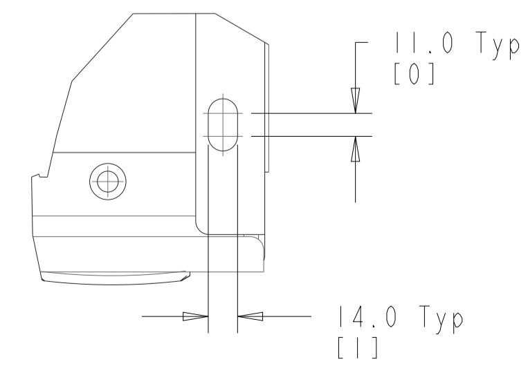
DETAIL A SCALE 0.400
