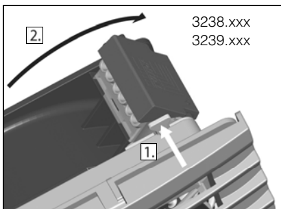
Fig. 4: Release the bayonet connection
