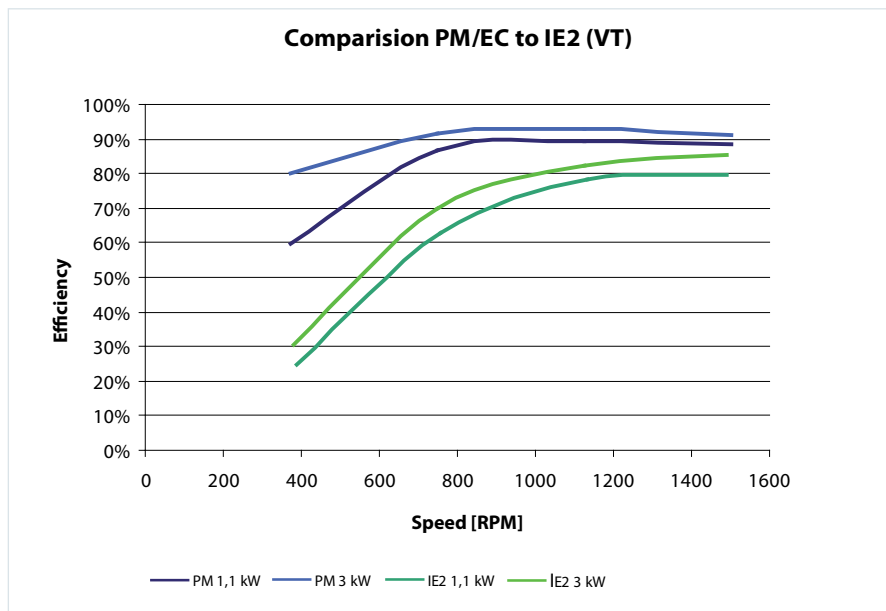
The diagram shows values measured by an independent university. Losses for the required control electronics are included in the figures.
