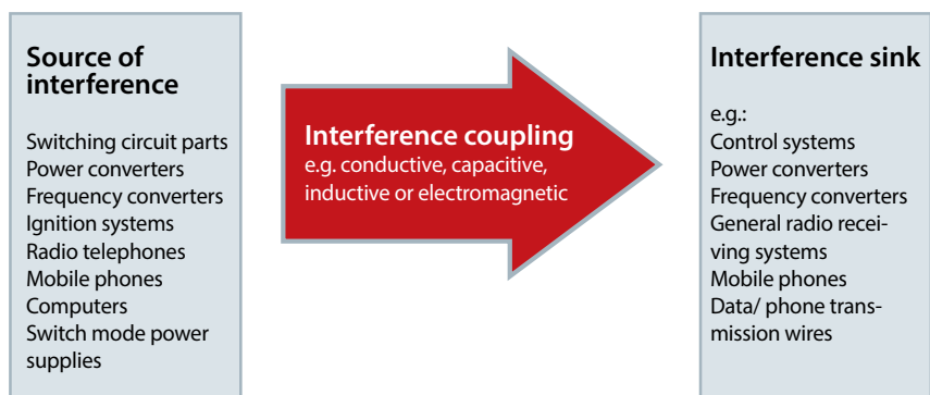
Overview of coupling paths for electromagnetic interference and typical examples
