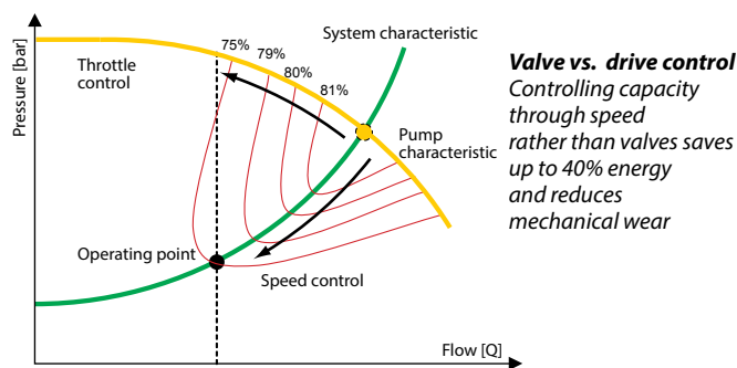
In addition to the pump and system characteristics, the graph also shows efficiency lines. Both throttle control and speed control cause the operating point to move out of the optimum efficiency range.
