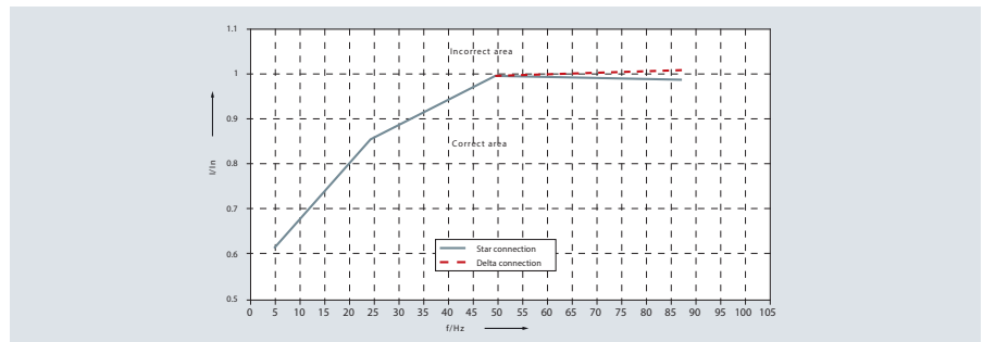
Variable speed current limitation, from the EC type-examination certificate of the Ex e motor. Enter the relevant information from the motor nameplate into the control panel of the drive. Then the drive will calculate max. current in relation to the motor speed. The curve represents the limit under which the current must be kept to prevent overheating of the motor. The nodes for the curves are determined by measurement from the Ex notified body. With a second protective device like the MCB 112, direct temperature monitoring is possible via a triple PTC thermistor circuit. Direct temperature monitoring also detects malfunctions such as blocked ventilation or inadmissibly high ambient temperatures.
