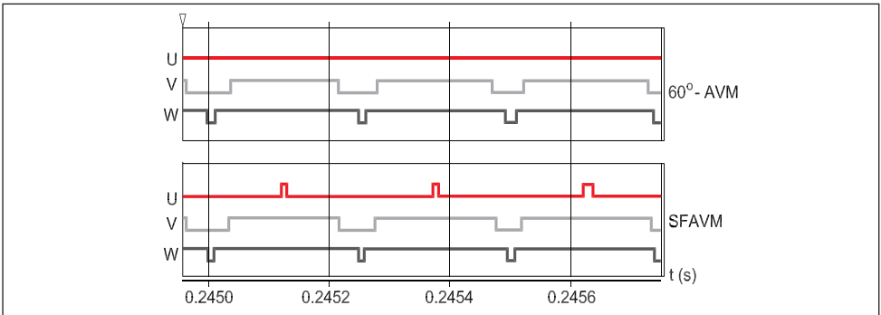
Fig. 2.18 Switching sequence of the 60° AVM and SFAVM methods for a number of 60° intervals
