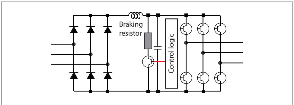
Fig. 3.11 Brake “chopper” and resistor
