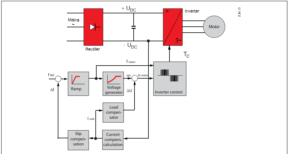
Fig. 2.22 Structure Scalar type Frequency Converter with compensation
