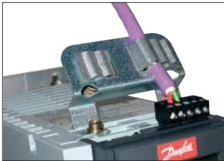
Fig. 8.5 Fieldbus connection
