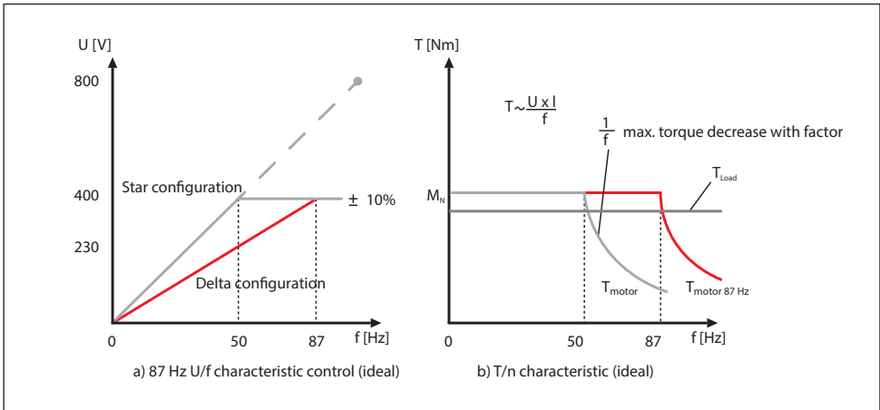
Fig. 3.2 87 Hz characteristic
