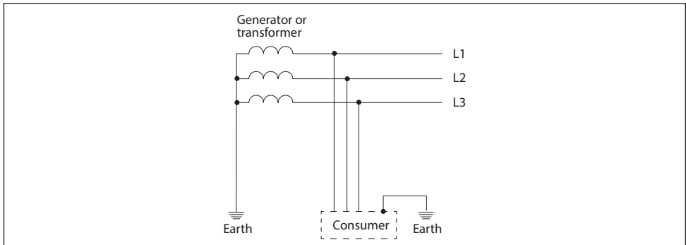
Fig. 6.5 IT system: Isolated mains; the neutral conductor may be earthed via an impedance or unearthed
