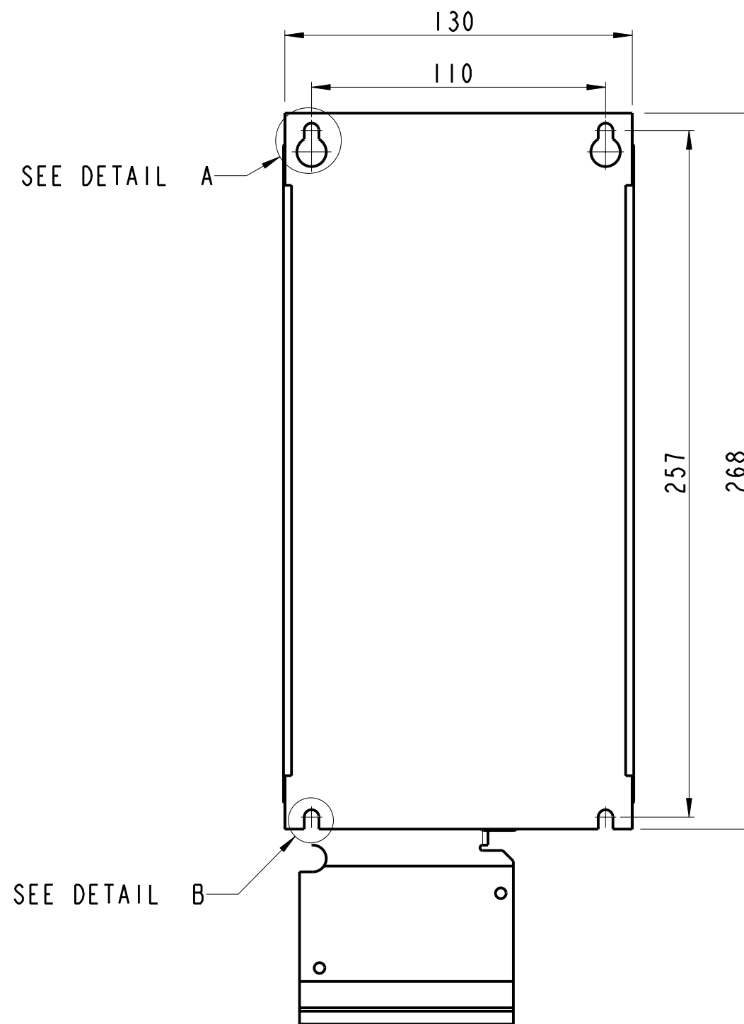
MOUNTING BASE
