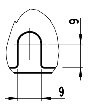
DETAIL B SCALE 1:1
