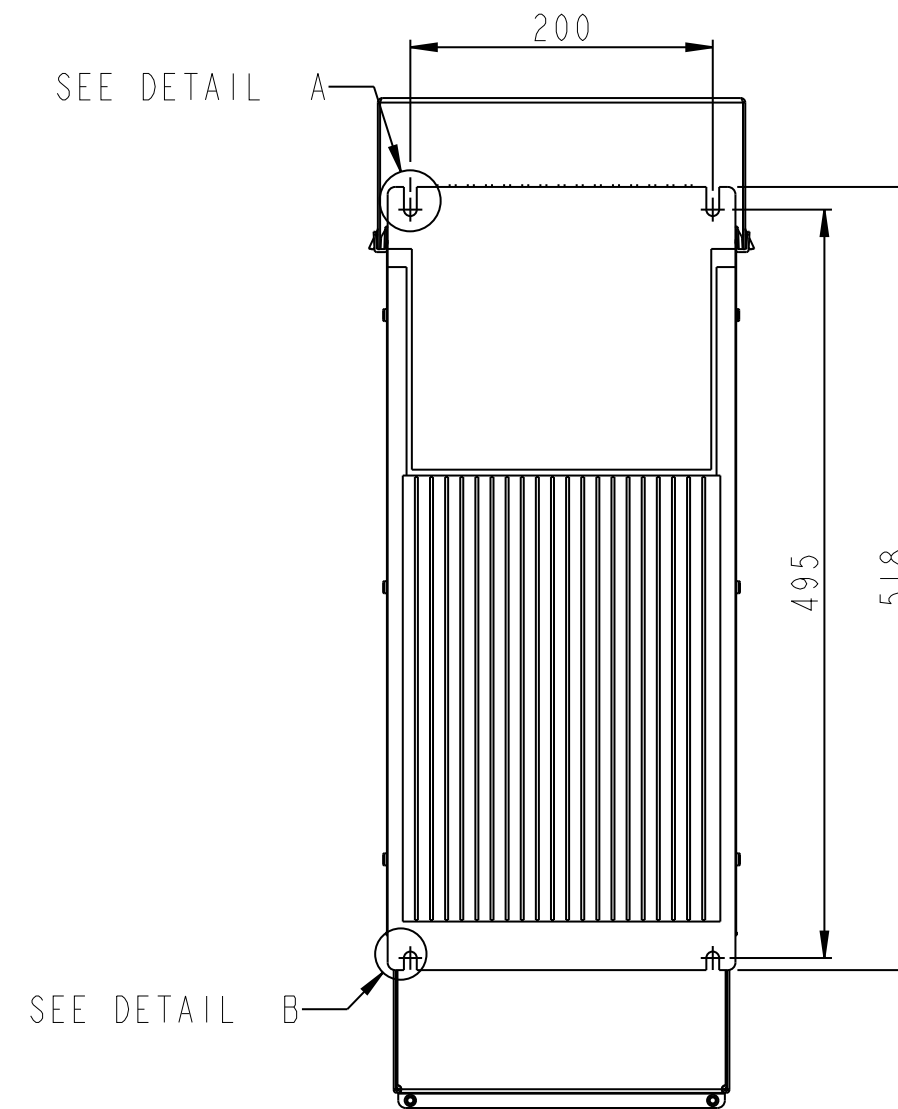
MOUNTING BASE
