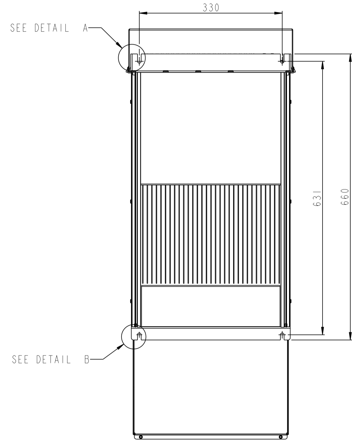
MOUNTING BASE
