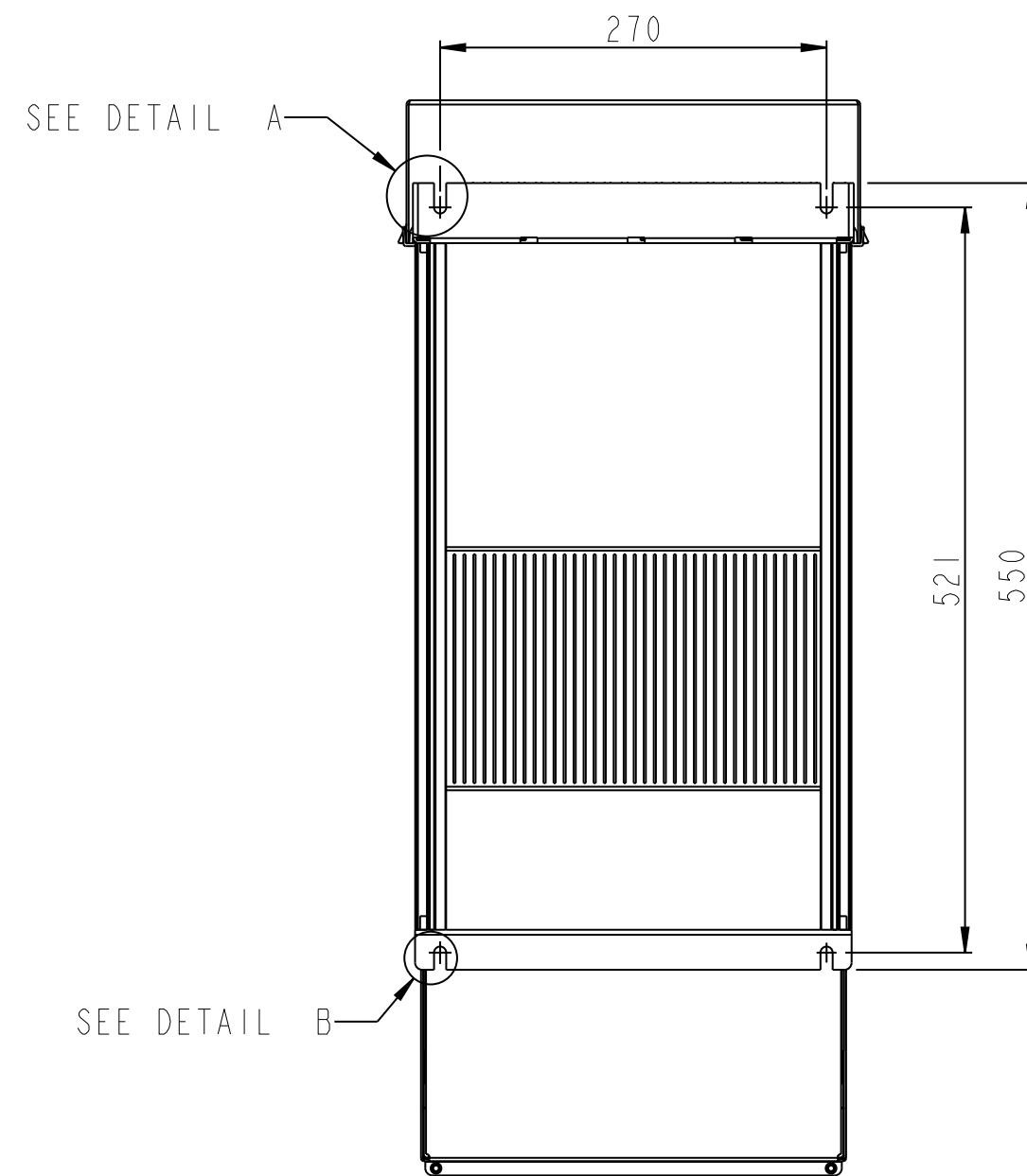
MOUNTING BASE
