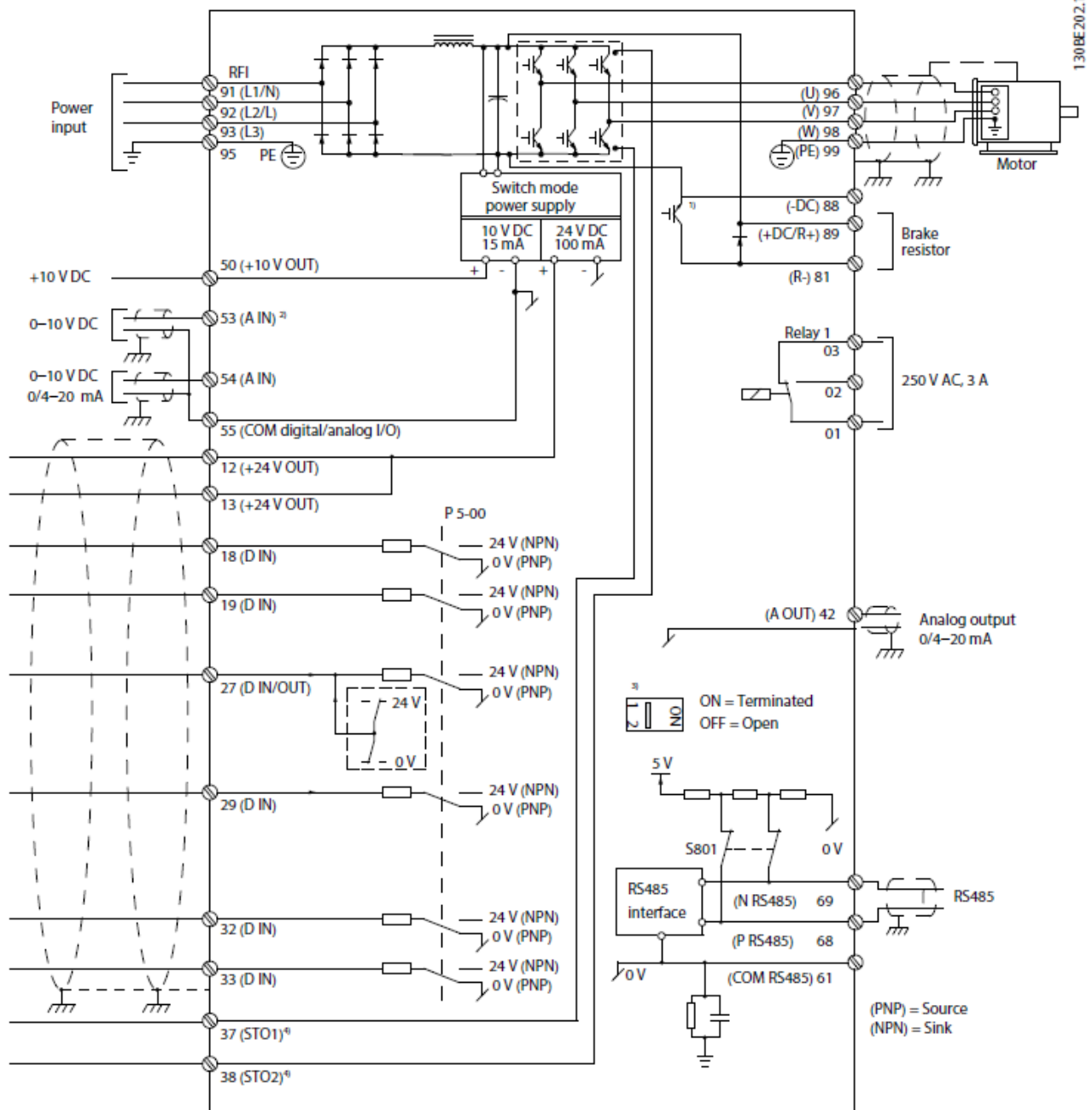
Illustration 2.1 Basic Wiring Schematic Drawing
