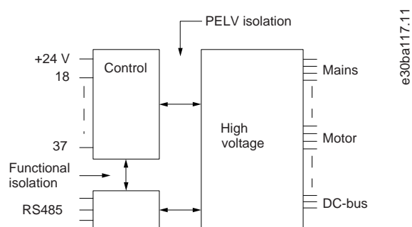
Illustration 71: Isolation PELV
