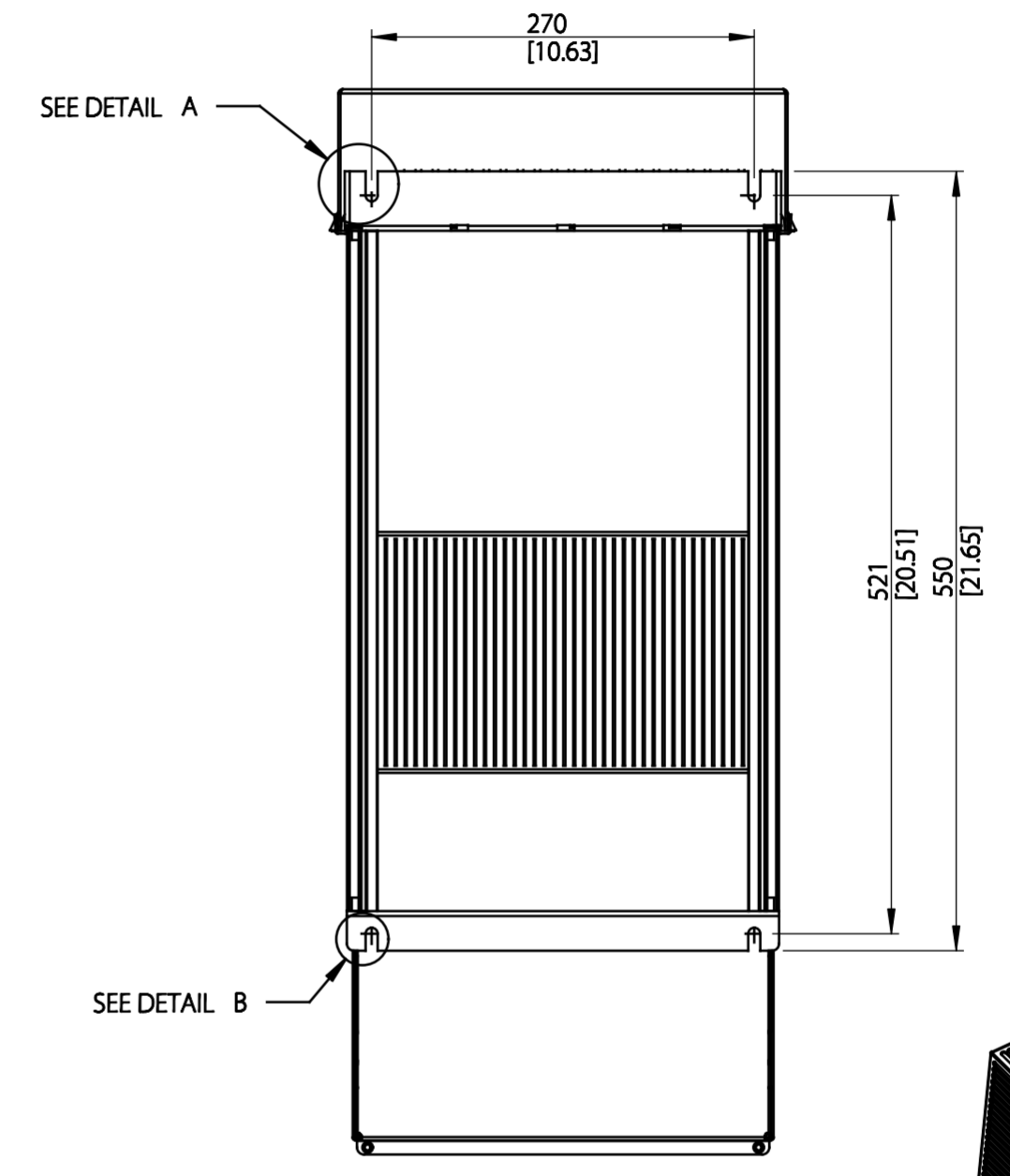
MOUNTING BASE
