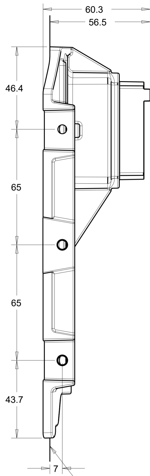
BASELINE MOTOR CABLE TERMINAL BOX
