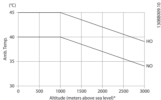
Illustration 3.13 Derating of Output Current versus Altitude at T_{AMB, MAX}
