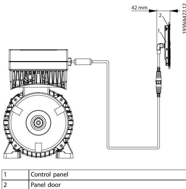
Illustration 3.10 LCP Remote Mounting
