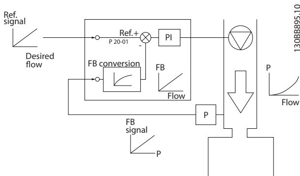
Illustration 2.17 Feedback Conversion
