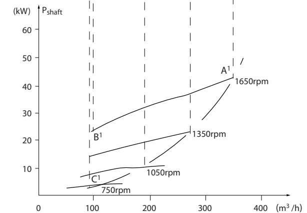
Illustration 4.10 Pump Performance
