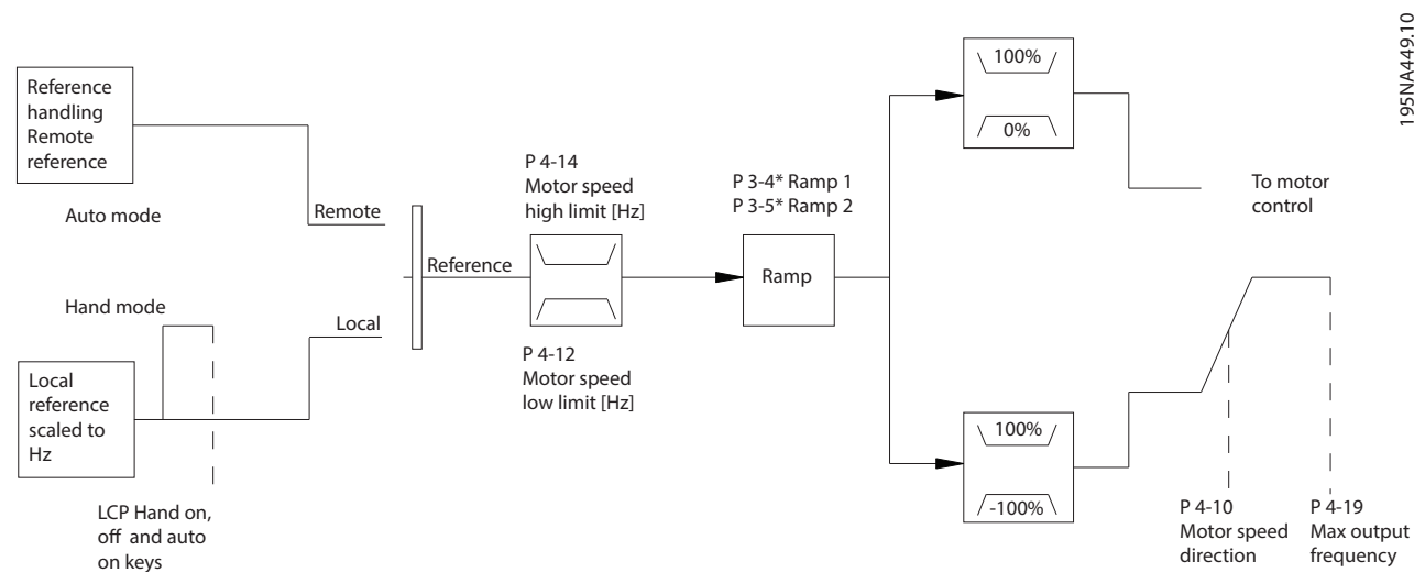
Illustration 2.13 Open-loop Structure
