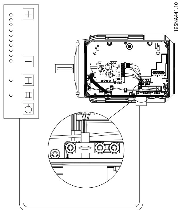
Illustration 3.11 LOP Connections
