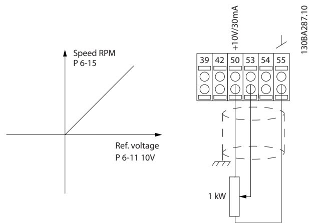
Illustration 4.4 Potentiometer Reference
