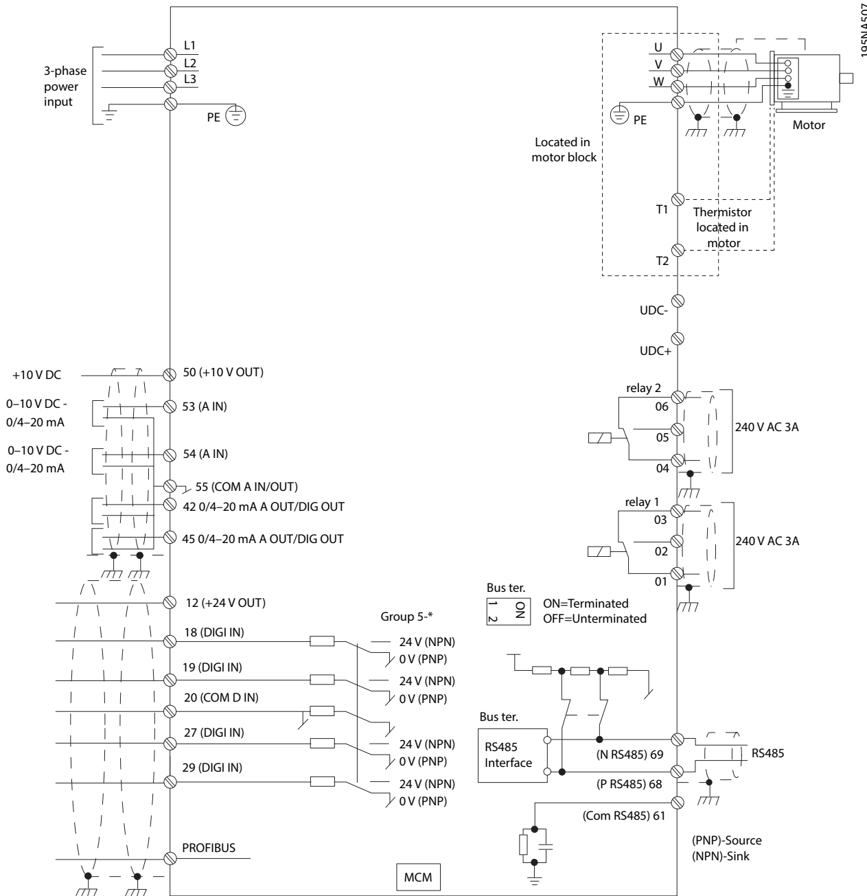
Illustration 2.4 Electrical Overview
