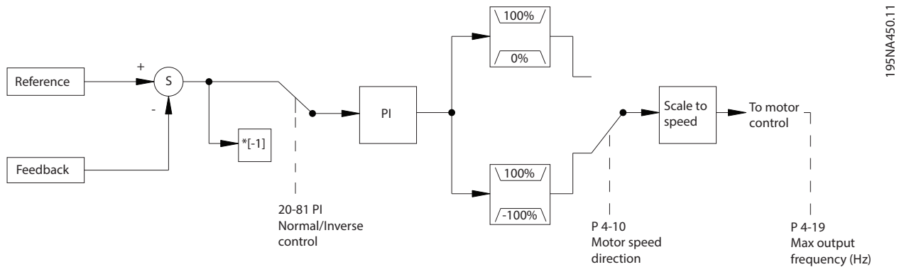
Illustration 2.14 Closed-loop Controller
