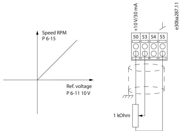
Illustration 4.4 Potentiometer Reference
