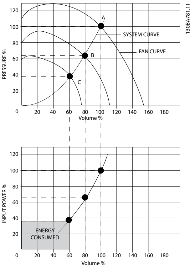
Illustration 4.6 Energy Savings at Reduced Fan Capacity
