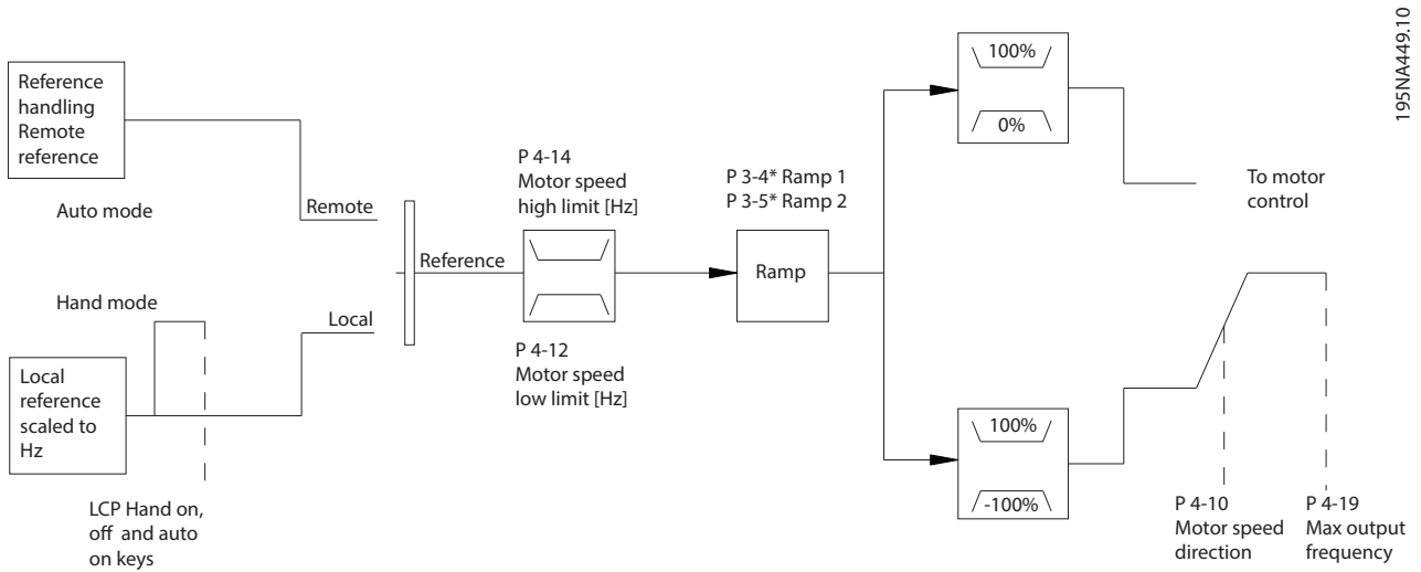
Illustration 2.13 Open-loop Structure
