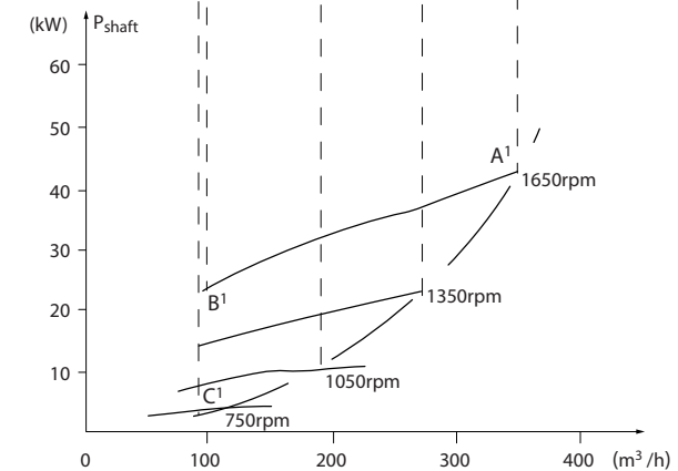
Illustration 4.10 Pump Performance
