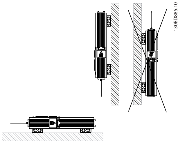
Illustration 9.11 Mechanical Mounting
