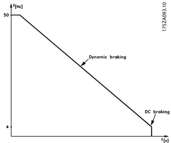
Illustration 7.1 Optimum Braking
