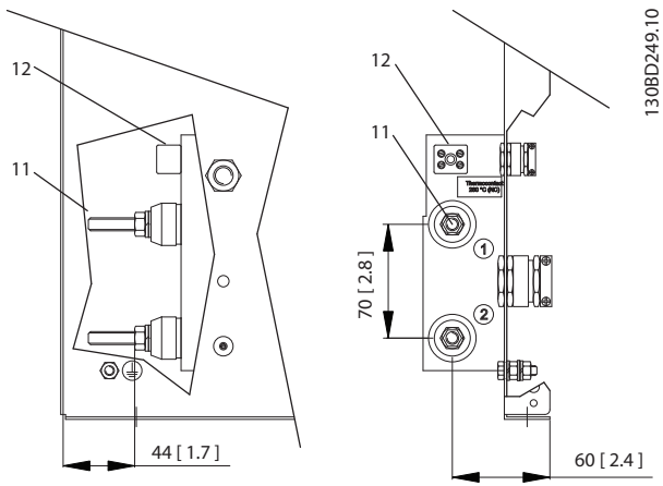
Illustration 9.52 Connections
