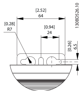
Illustration 9.9 Mounting Hole
