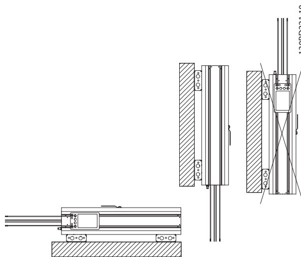
Illustration 9.28 Mechanical Mounting
