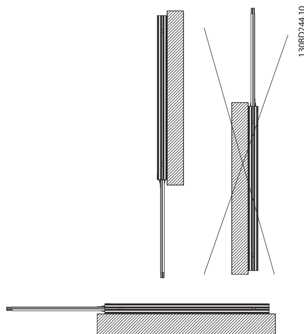
Illustration 9.38 Mechanical Mounting
