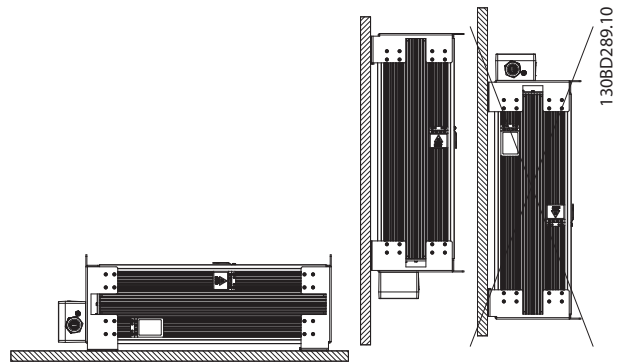
Illustration 9.90 Mechanical Mounting
