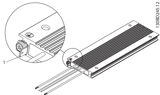
Illustration 2.3 Flat-pack IP54
