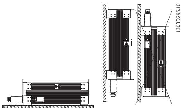
Illustration 9.84 Mechanical Mounting
