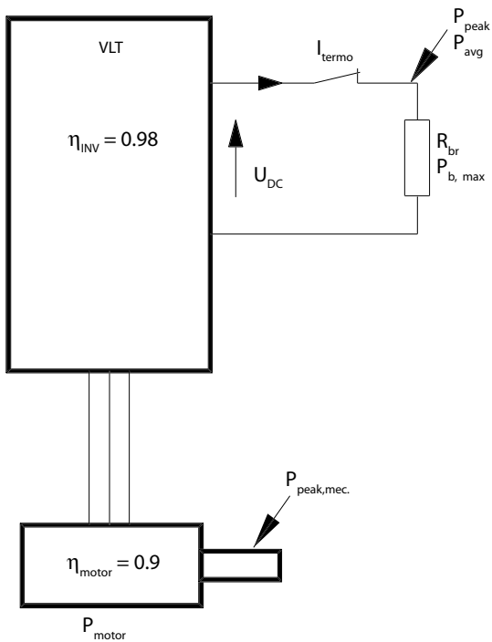
Illustration 4.1 Brake Set-up
