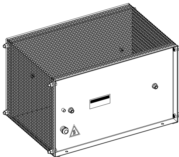
Illustration 2.7 Steel Grid House IP20
