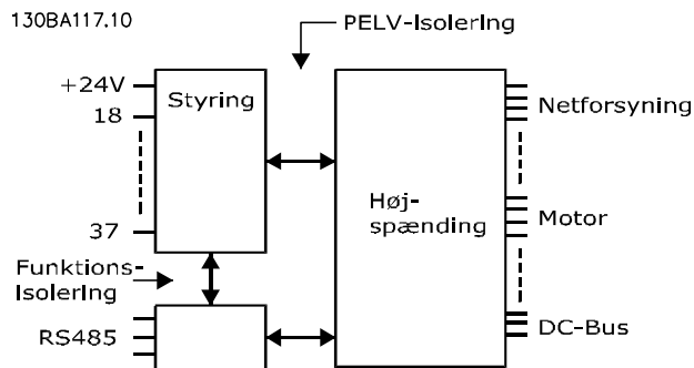
Illustration 8.1 PELV-isolering
