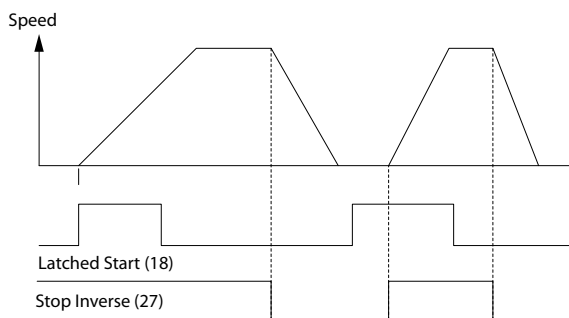
Illustration 6.3 Pulsstart/inverteret stop
