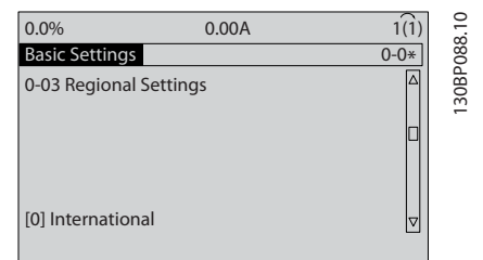
Illustration 5.4 Basisindstillinger
