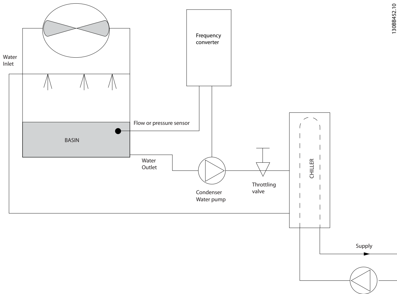
Illustration 5.19 Drive Used with a Condenser Pump
