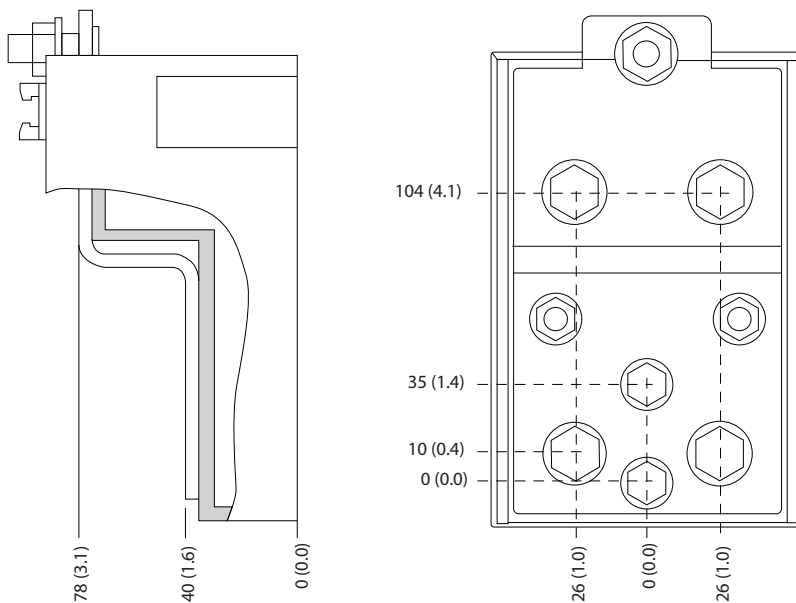
Illustration 8.12 Detailed Terminal Dimensions for E1/E2
