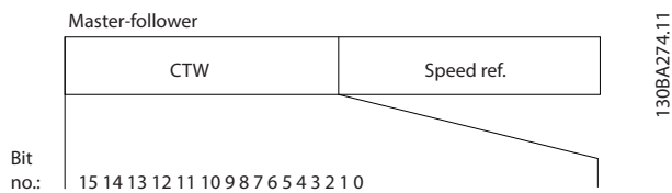
Illustration 14.16 CW Master-to-Slave
