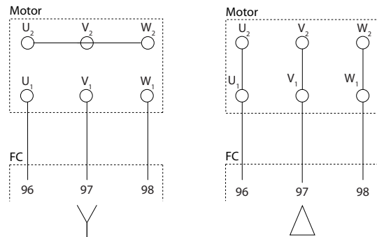
Illustration 10.5 Motor Cable Connection
