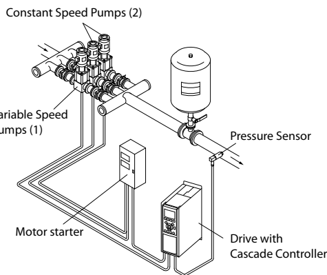
Illustration 5.22 Basic Cascade Controller
