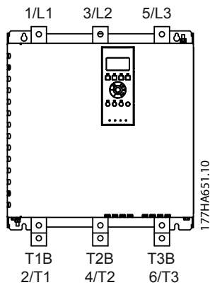
Abbildung 4.7 Bypass-Klemmen am MCD5-0245C, 245 A
