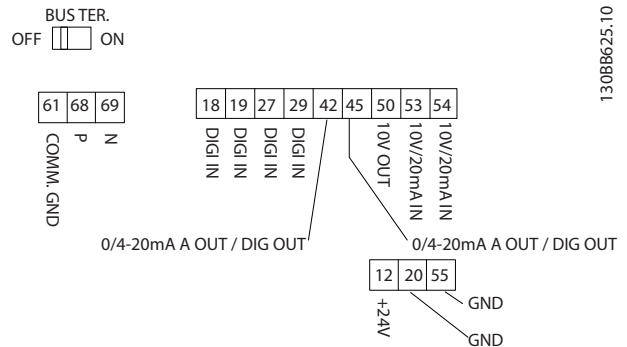
Figure 1.24 Control Terminals
