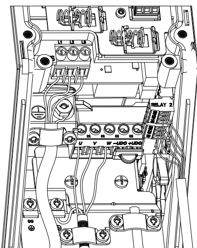
Illustration 3.16 IP54 I2-I3-I4-kapsling
