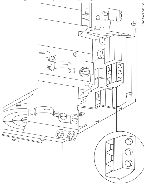
Illustration 3.12 H10-kapsling IP20, 600 V, 11-15 kW (15-20 hk)
