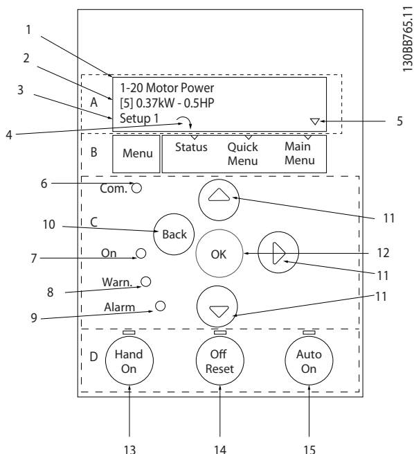
Illustration 4.1 LCP-betjeningspanel
