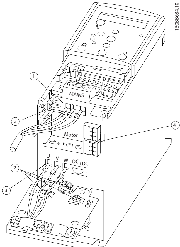
Illustration 3.4 Kapslingsstørrelse H6 IP20, 380–480 V, 30–45 kW (40–60 hk) IP20, 200–240 V, 15–18,5 kW (20–25 hk) IP20, 525–600 V, 22–30 kW (30–40 hk)
