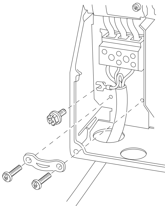
Figure 5.16 I6 Frame IP54 380-480 V 30-50 hp [22-37 kW]
