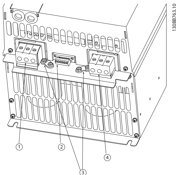
Figure 5.4 H7 Frame
