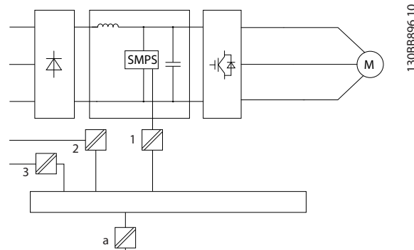
Figure 2.25 Galvanic Isolation
