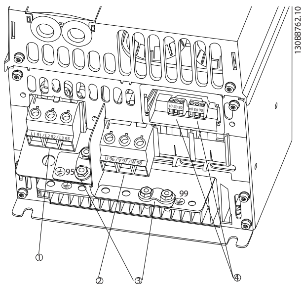
Figure 5.3 H6 Frame
