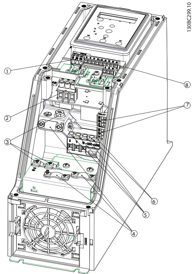
Figure 5.12 I2 Frame IP54 380–480 V 1–5 hp [0.75–4.0 kW]
