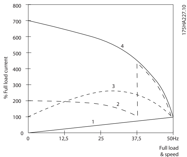
Figure 2.8 Start-up Current
