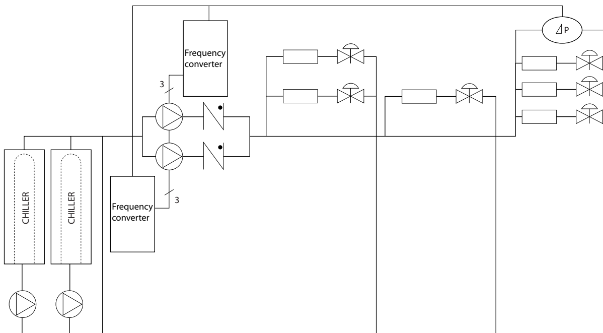
Figure 2.16 Secondary Pumps
