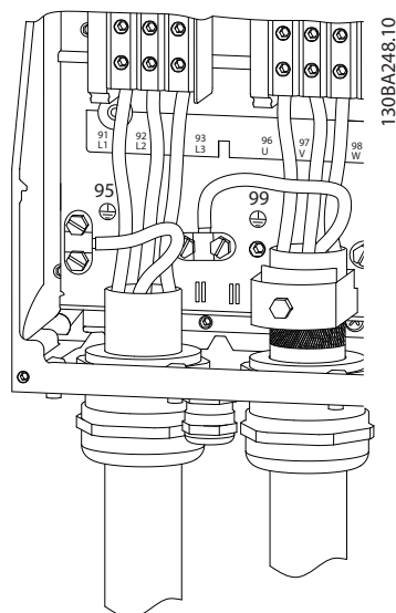
Figure 5.19 I7, I8 Frame IP54 380–480 V 60–75 hp [45–55 kW] IP54 380–480 V 100–125 hp [75–90 kW]
