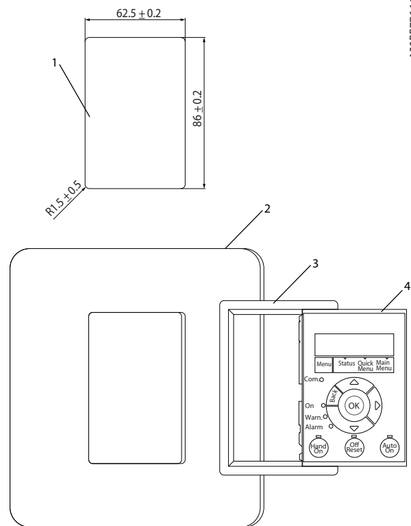
Figure 3.2 Place LCP on Panel
