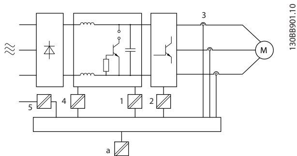
Figure 2.26 Galvanic Isolation
