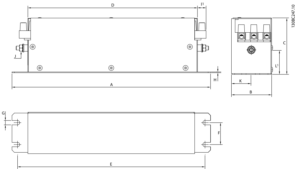
Figure 4.2 RFI Filter
