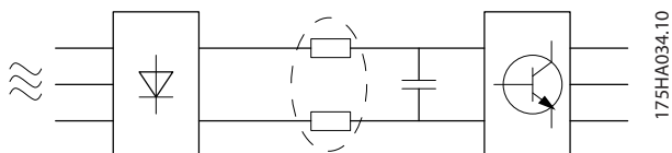
Figure 2.24 Harmonic Currents
