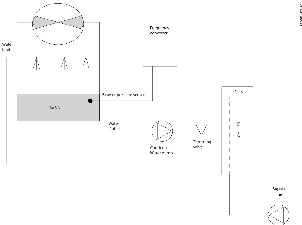
Figure 2.14 Condenser Pumps
