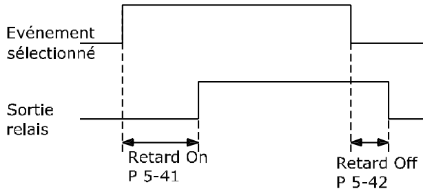
Illustration 3.26 Relais, retard OFF
