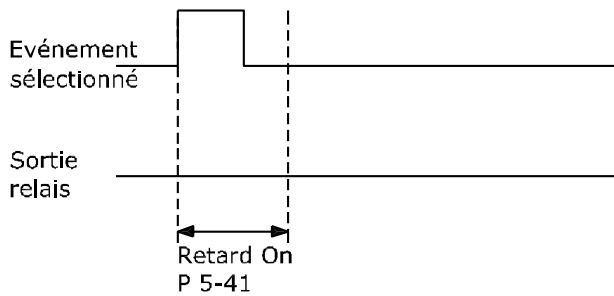
Illustration 3.25 Relais, retard ON
