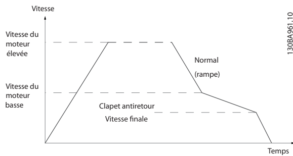
Illustration 3.20 Rampe clapet anti-retour
